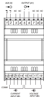
Fig.3 Front View of Device for electrical Connections
