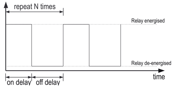
De-energized configuration
