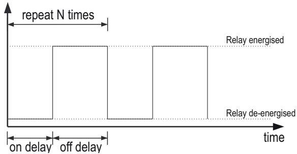
Energized configuration
