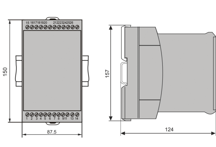
Fig. 6. MXX in housing T24 clipped onto a top-hat rail (35 X 15 mm or 35 X 7.5 mm, acc. to EN 50 022).
