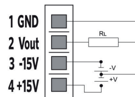
Fig. 1.2: Connection Diagram
