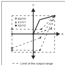
Bent characteristic
