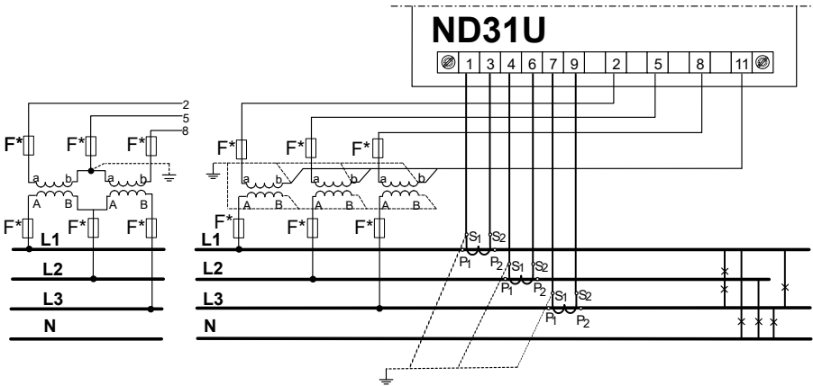
Fig.6.Connections of input signals in three-phase 4-wire network
