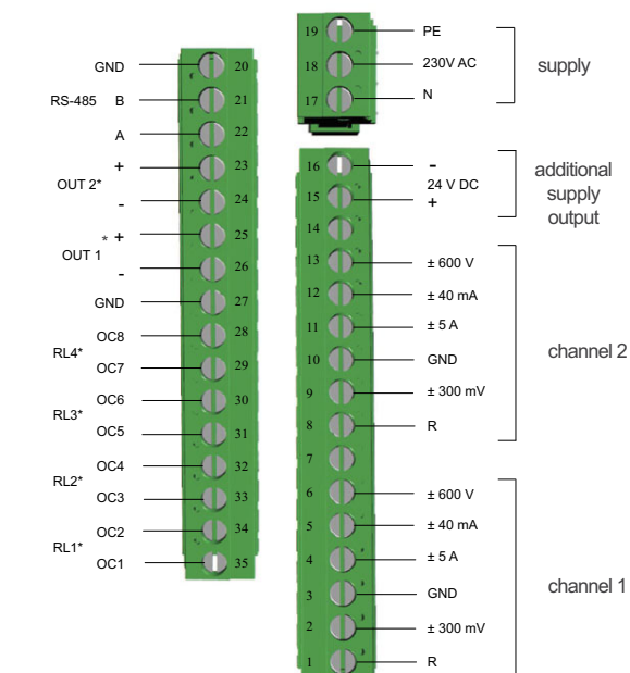
Fig. 1 Description of the terminal strip.
