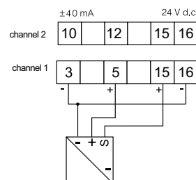
three-wire object transducer
