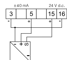
three-wire object transducer
