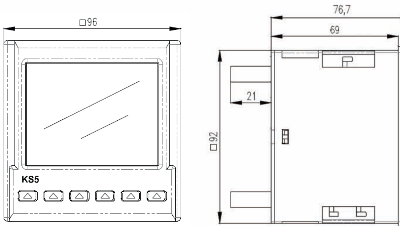
Fig.3. Overall dimensions of KS5 meter
