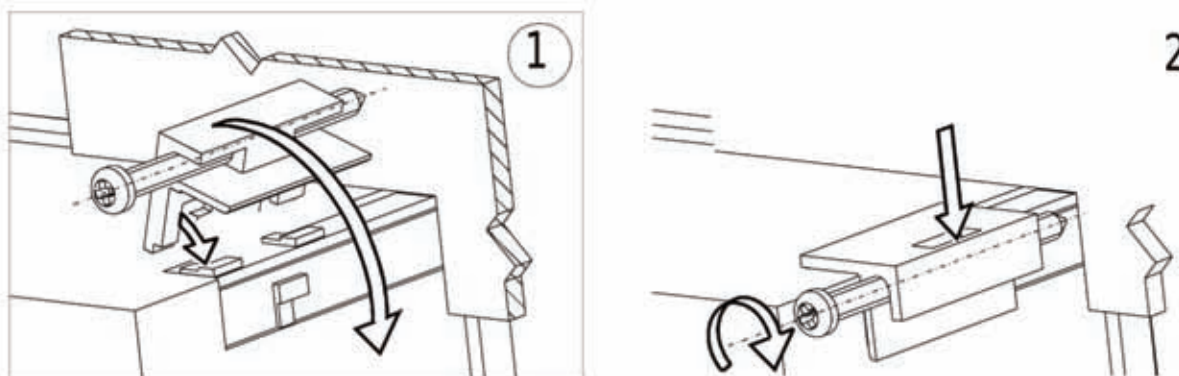
Fig.2. Meter fixing
