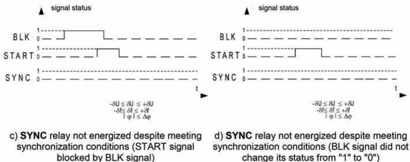
Fig.14, Graphic illustration of BLK and START input signals control with SYNC synchronization relay
