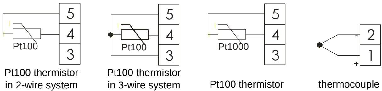
Fig. 4: Input signals
