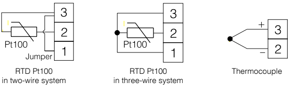
Fig. 4. Connection of input signals
