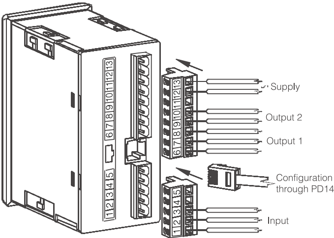
Fig. 3. View of controller connection strips
