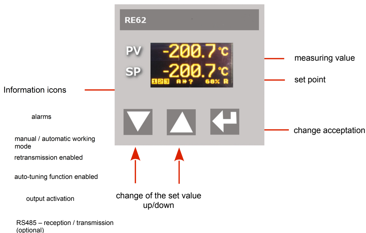
Figure 6. RE62 controller panel description
