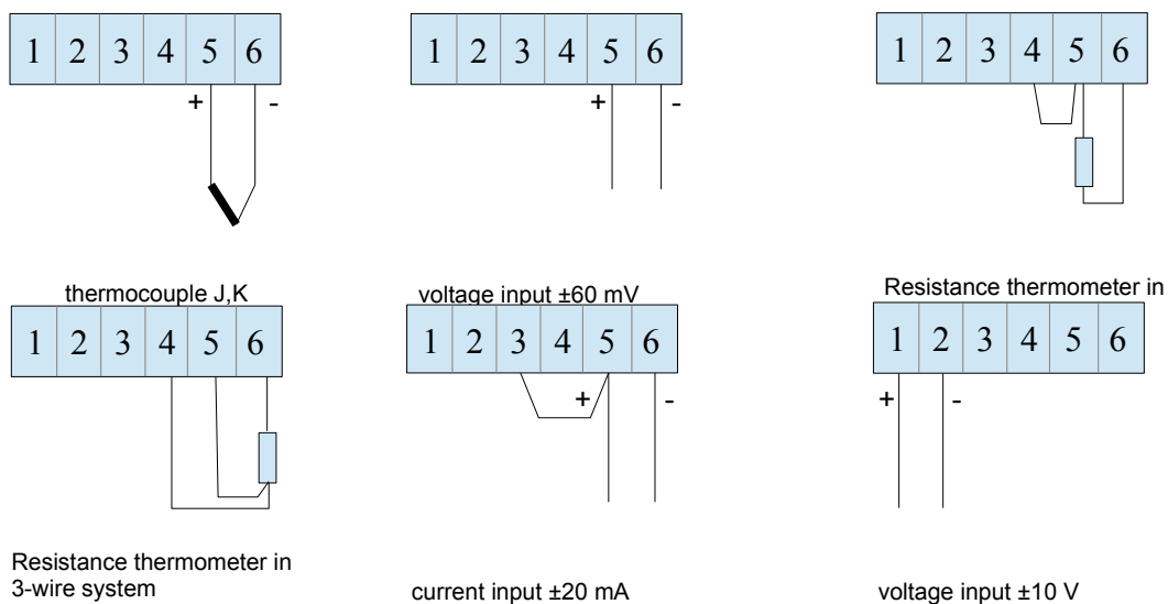
Figure 4. Connections of measuring signals
