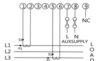
3 Phase 3 wire Unbalanced load
