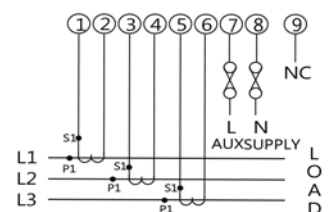
3 Phase 4 wire Unbalanced load
