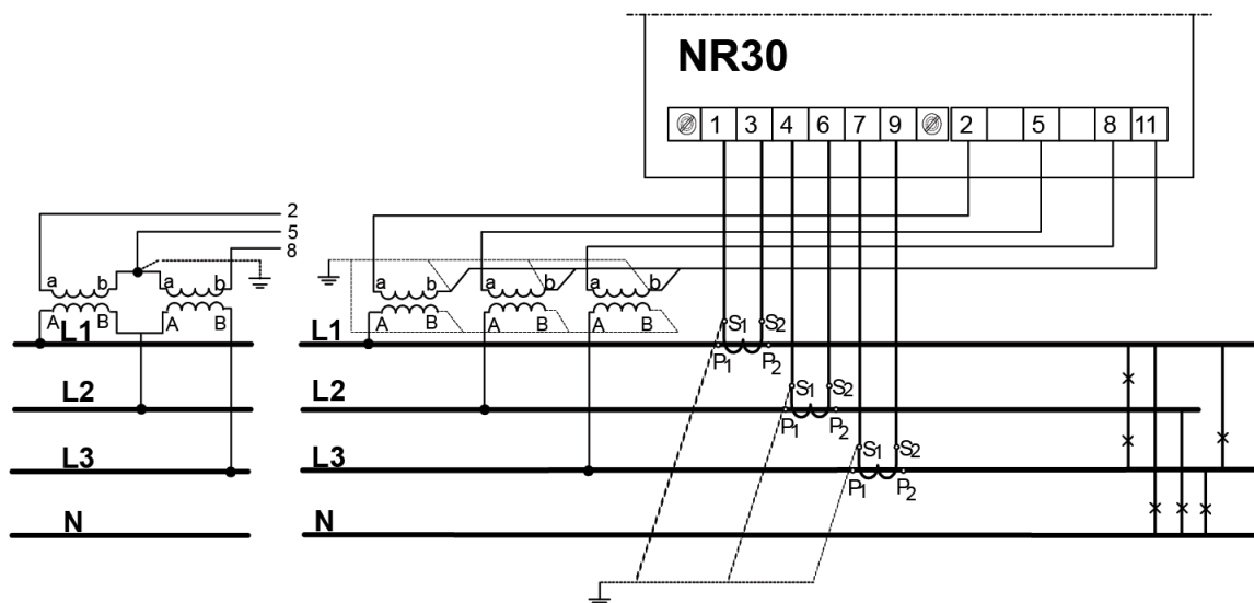
Fig.5. Input signal connection in 3-phase 4 - wire network
