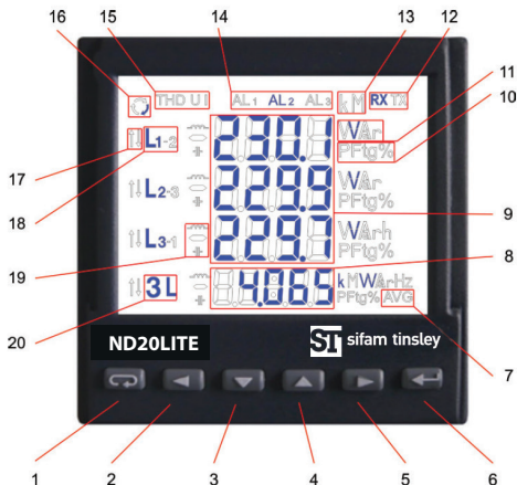
Fig 4. Frontal panel
