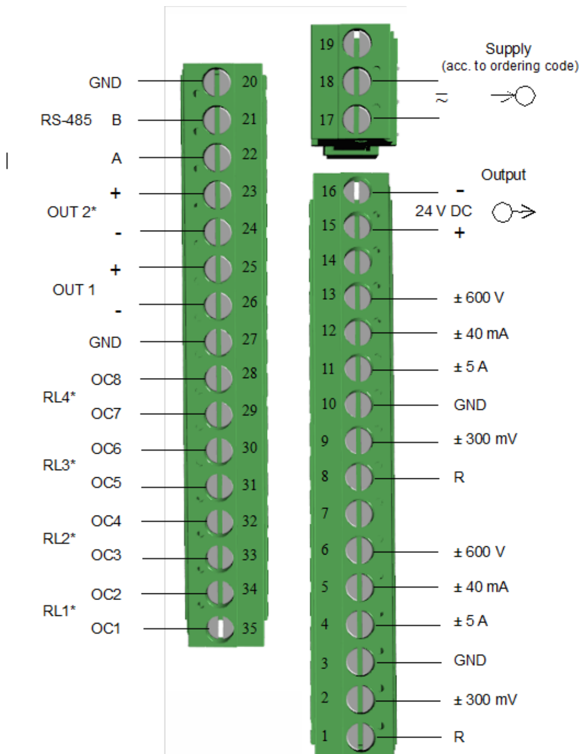
Fig. 3: Electrical connections of NA6Plus meter
