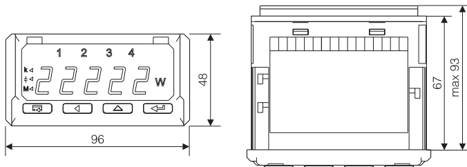
Fig. 3. Overall dimensions
