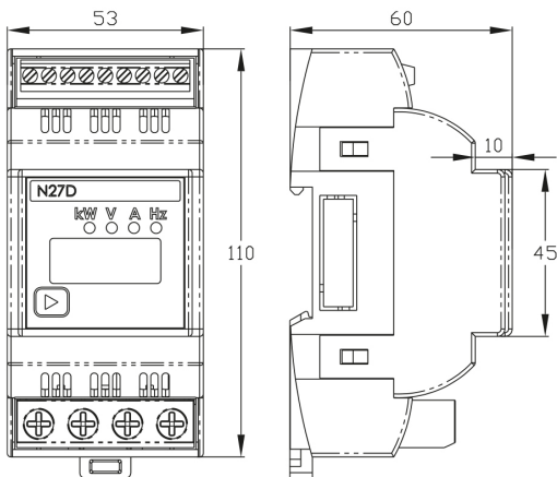
Fig. 2. Overall dimensions
