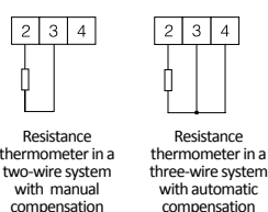
Fig. 1. Electrical connections of the N25S meter
