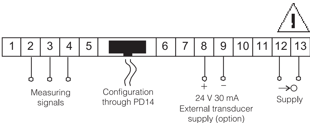
Fig. 4. Electrical connection of the N24T, N25T meters
