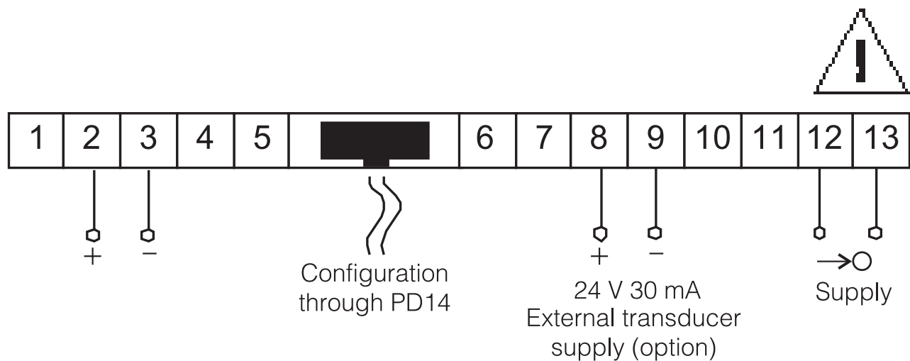
Fig. 3. Electrical connection of the N24S, N25S meters
