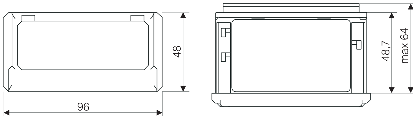
Fig. 2. Overall dimensions
