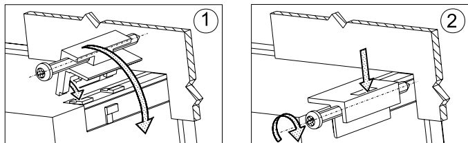
Fig. 1. N20Z and N20ZPLUS meter fixing.
