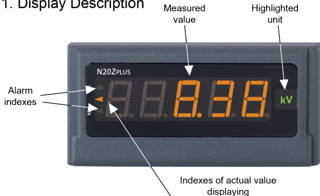
Fig. 7. Frontal panel
