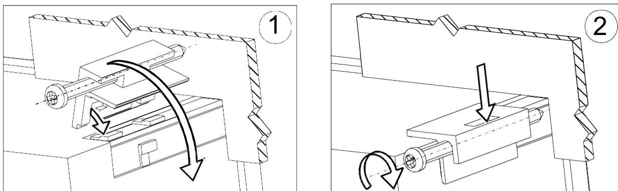
Fig.2 Recorder mounting
