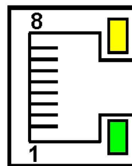
Fig.32. View and pin numbering of the recorder RJ45 socket
