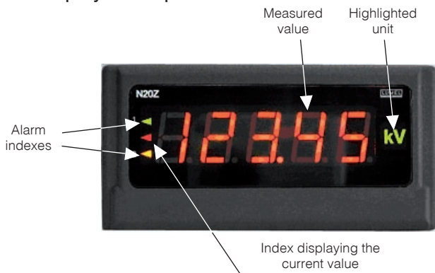
Fig. 5 frontal panel
